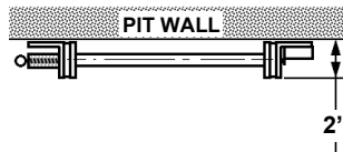
TOP VIEW - LADDER FOLDED
