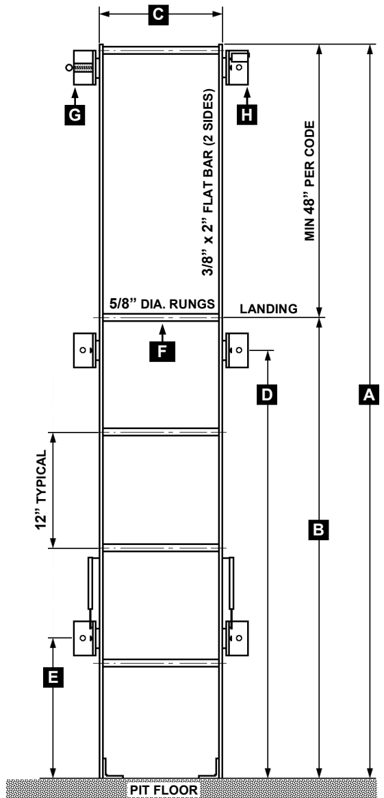
FRONT VIEW - LADDER UNFOLDED
