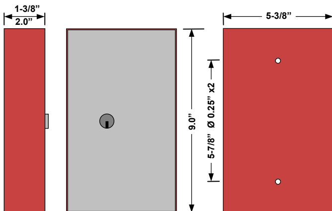
KB, FKB Surface mount, 9"H x 5-3/8"W", 1-3/8" or 2" deep
