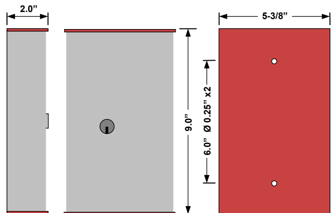
SKB Surface mount, 9"H x 5-3/8"W", 2" deep
