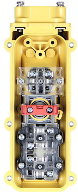
Wiring. Pendant station Model PS-824.
