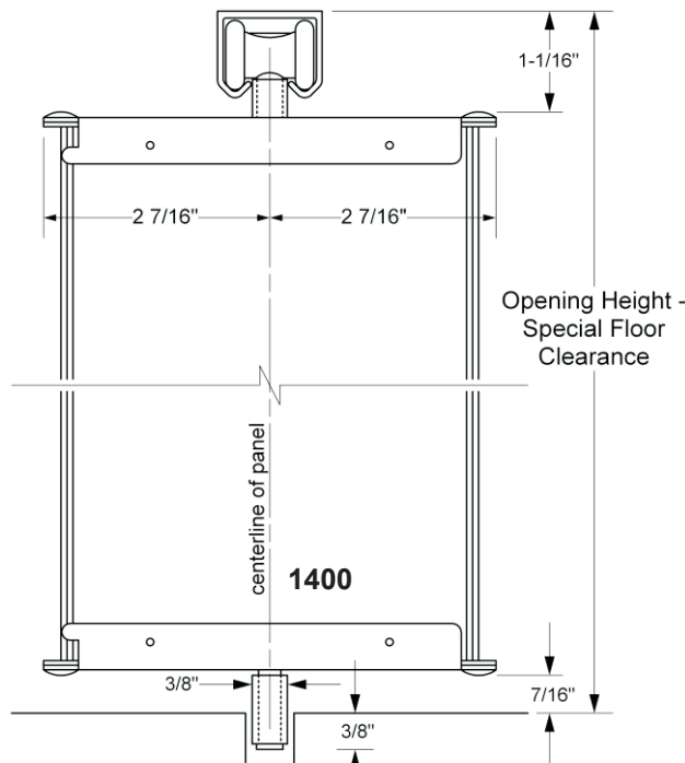
Opening Height with Special Floor Clearance
